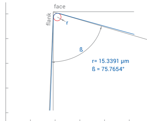
The measurement log shows the surface quality of the edge rounding in the μm range.
